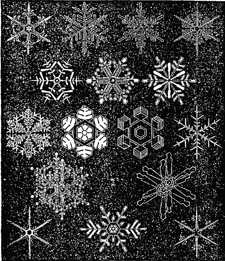
Snow crystals (enlarged). After Glaisher. Illustration from M. Wilh. Meyer, "The forces of nature"
