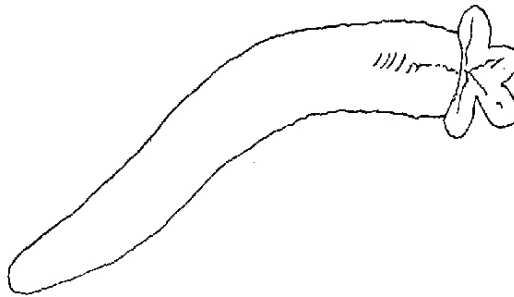
Outline of the comet shape of Ophidiaster multiforis .
